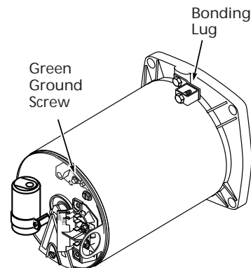
Figure 4 - Typical ground screw and bonding lug locations.
