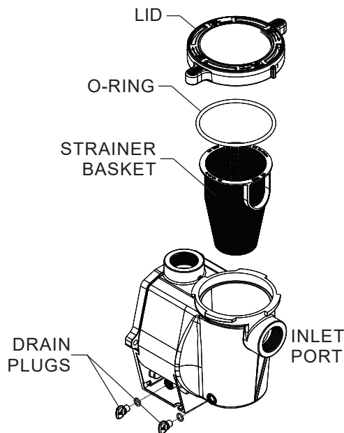
Strainer Pot Assembly
