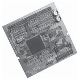
AquaLink RS Power Center Firmware CPU PCB (Rev N or Later)
