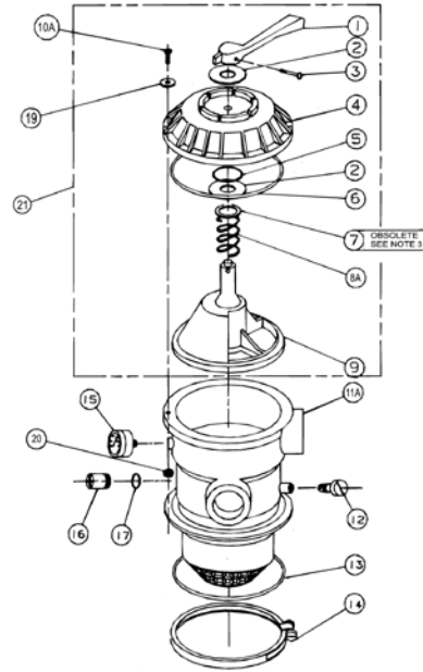
For (262506) Clamp Style Valve For TA-D Filters
