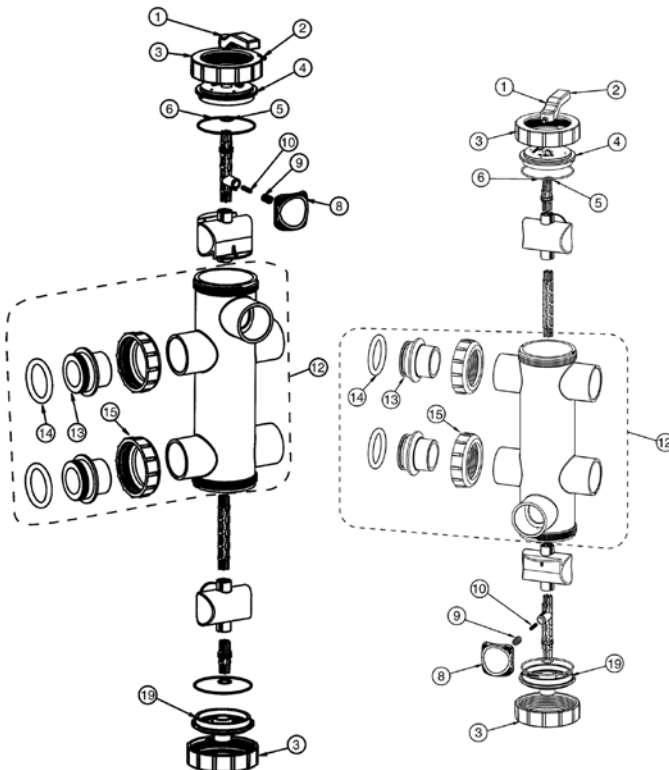
FullFlow Sand Valve 263011 7.5" Centerline Filters
