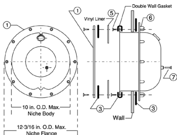
Standard 10 Hole Pattern for vinyl or fiberglass
