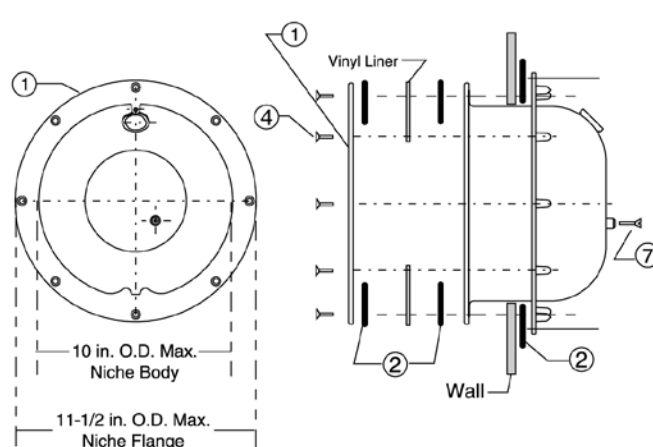
American 8 Hole Pattern
