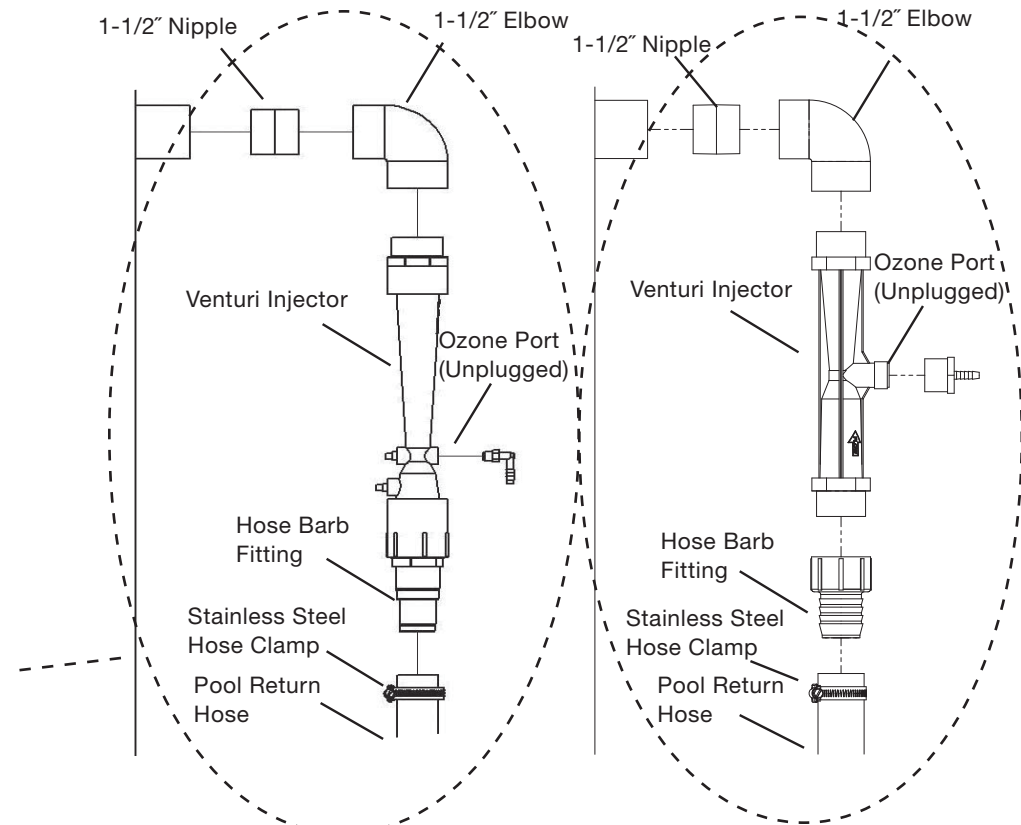
Figure 2b Mazzei Injector Assembly Exploded View
