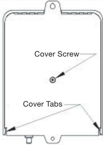
Figure 3 Cover screw and tabs
